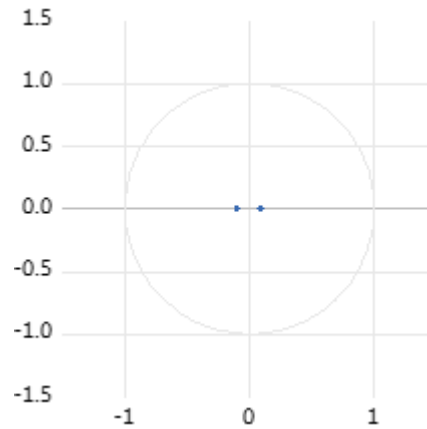
Figure 1: AR root graph.
